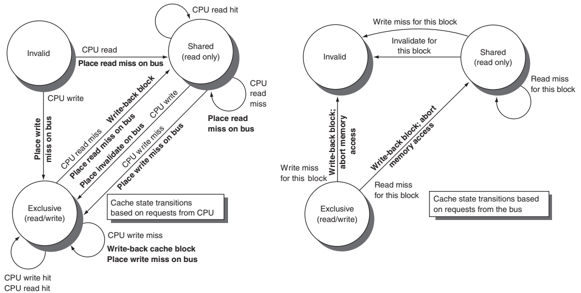
FIGURE 5.12.10 A write-invalidate, cache-coherence protocol for a write-back cache, showing the states and state transitions for each block in the cache. The cache states are shown in circles, with any access permitted by the processor without a state transition shown in parentheses under the name of the state. The stimulus causing a state change is shown on the transition arcs in regular type, and any bus actions generated as part of the state transition are shown on the transition arc in bold. The stimulus actions apply to a block in the cache, not to a specific address in the cache. Hence, a read miss to a block in the shared state is a miss for that cache block but for a different address. The left side of the diagram shows state transitions based on actions of the processor associated with this cache; the right side shows transitions based on operations on the bus. A read miss in the exclusive or shared state and a write miss in the exclusive state occur when the address requested by the processor does not match the address in the cache block. Such a miss is a standard cache replacement miss. An attempt to write a block in the shared state generates an invalidate. Whenever a bus transaction occurs, all caches that contain the cache block specified in the bus transaction take the action dictated by the right half of the diagram. The protocol assumes that memory provides data on a read miss for a block that is clean in all caches. In actual implementations, these two sets of state diagrams are combined. In practice, there are many subtle variations on invalidate protocols, including the introduction of the exclusive unmodified state, as to whether a processor or memory provides data on a miss.
