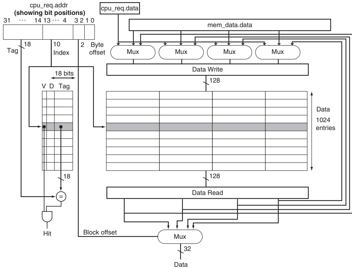
FIGURE 5.12.3 Block diagram of the simple cache using the Verilog names. Not shown are the write enables for the cache tag memory and for the cache data memory, or the control signals for multiplexers that supply data for the Data Write variable. Rather than have separate write enables on every word of the cache data block, the Verilog reads the old value of the block into Data Write and then updates the word in that variable on a write. It then writes the whole 128-bit block.
