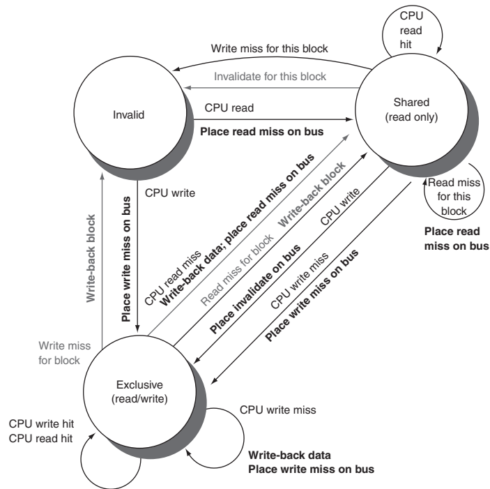
FIGURE 5.12.11 Cache coherence state diagram with the state transitions induced by the local processor shown in bold and by the bus activities shown in gray. As in Figure 5.12.10, the activities on a transition are shown in bold.
